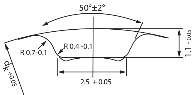
AT5-0 NO BACKLASH
