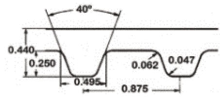
XH-Pitch
