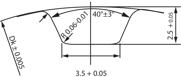
T10-0 No Backlash
