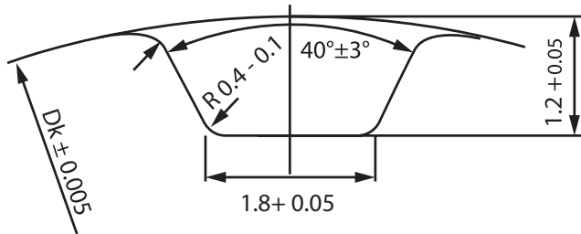
T5-0 No Backlash
