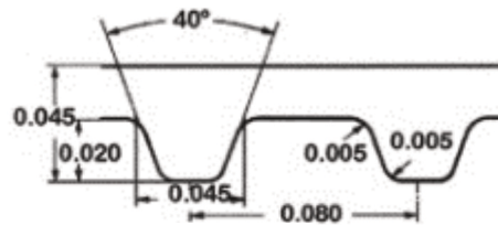
MXL-Pitch
