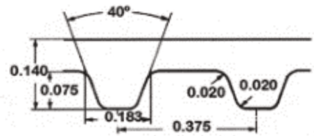
L-Pitch
