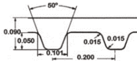
XL-Pitch
