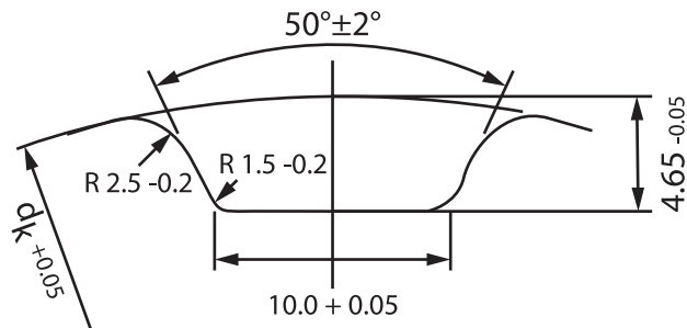
AT20-0 NO BACKLASH
