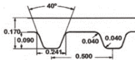
H-Pitch
