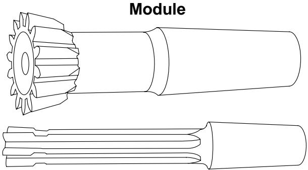
Module Maximum Tooth Chart 20° PA
