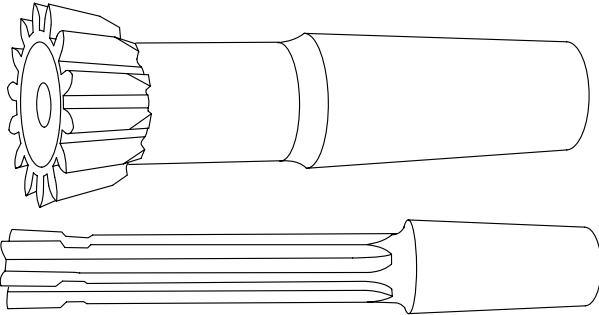
Maximum Tooth Chart 20° PA
